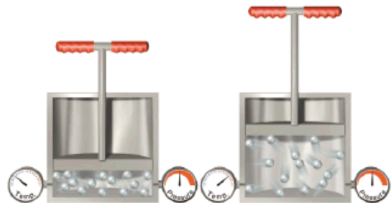
Lowering the temperature of the gas causes the particles to move more slowly. They hit the sides of the piston less often and with less force. As a result, the plunger enters the piston and the volume of the gas decreases.
