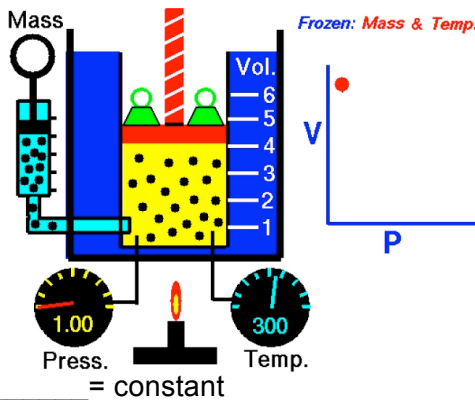
Lifting the plunger decreases the pressure of the gas. The particles of gas collide less often with the walls of the piston as they spread farther apart. The volume of the gas increases as the pressure decreases.
